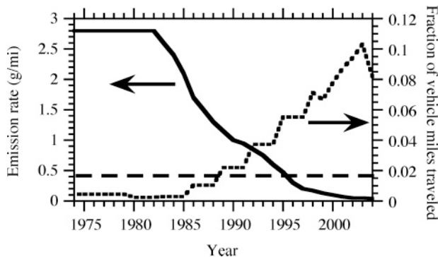
FIGURE 1. Vehicle-fleet-averaged hydrocarbon emission rate in 2003 (straight long-dashed line), determined from the frequency distribution of vehicle miles traveled versus vehicle age (30) and the hydrocarbon emission rate from several hundred thousand passenger vehicles and light-duty trucks in 2003 versus model year 1982–2004 (31). Emission rates prior to 1982 were held to the 1982 value. The ratio of the fleet-averaged emission rate (straight long-dashed line) to the 2004 model-year emission rate (last point of solid line) is about 10.4:1.
