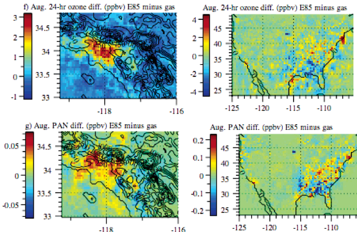
FIGURE 3. Modeled differences in the August 24-hour average near-surface mixing ratios of (a) ethanol, (b) acetaldehyde, (c) formaldehyde, (d) 1,3-butadiene, (e) benzene, (f) ozone, and (g) PAN in Los Angeles and the United States when all gasoline vehicles (in 2020) were converted to E85 vehicles under the emission assumption in Tables 1 and S4, respectively. Figures S1 and S5 gives difference plots and E85-alone plots for additional chemicals for Los Angeles and the U.S., respectively.
