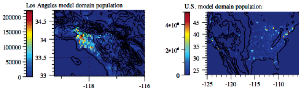
FIGURE 2. Population distributions of the (a) Los Angeles and (b) U.S. model domains (25, from U.S. 2000 census data). The total population in the Los Angeles domain was 17,267,158; that in the U.S. domain was 277,292,992. The California Air Resources Board estimates a population increase of 22.895% between 2000 and 2020 (29), giving estimated populations in 2020 in the respective domains of 21,220,474 and 340,779,223.
